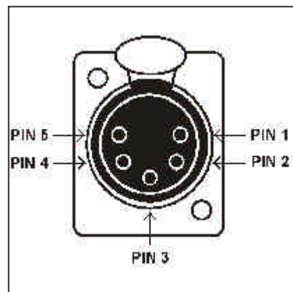
Figure 8 - 5: DMX Connector
