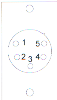
DMX In
